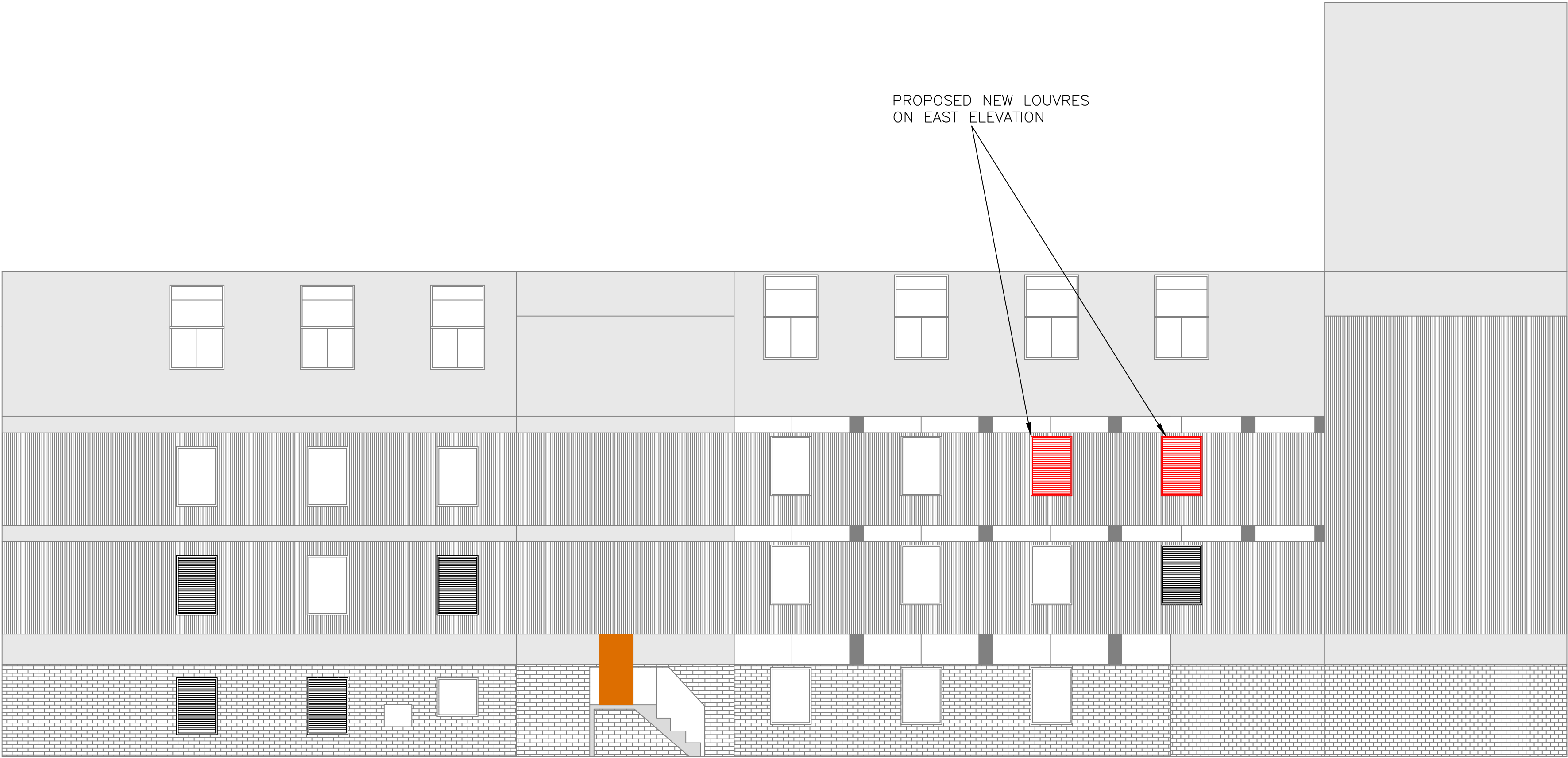
PROPOSED EAST ELEVATION (1:100)
