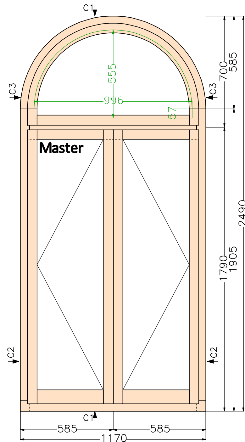
View from outside (scale 1:15)
