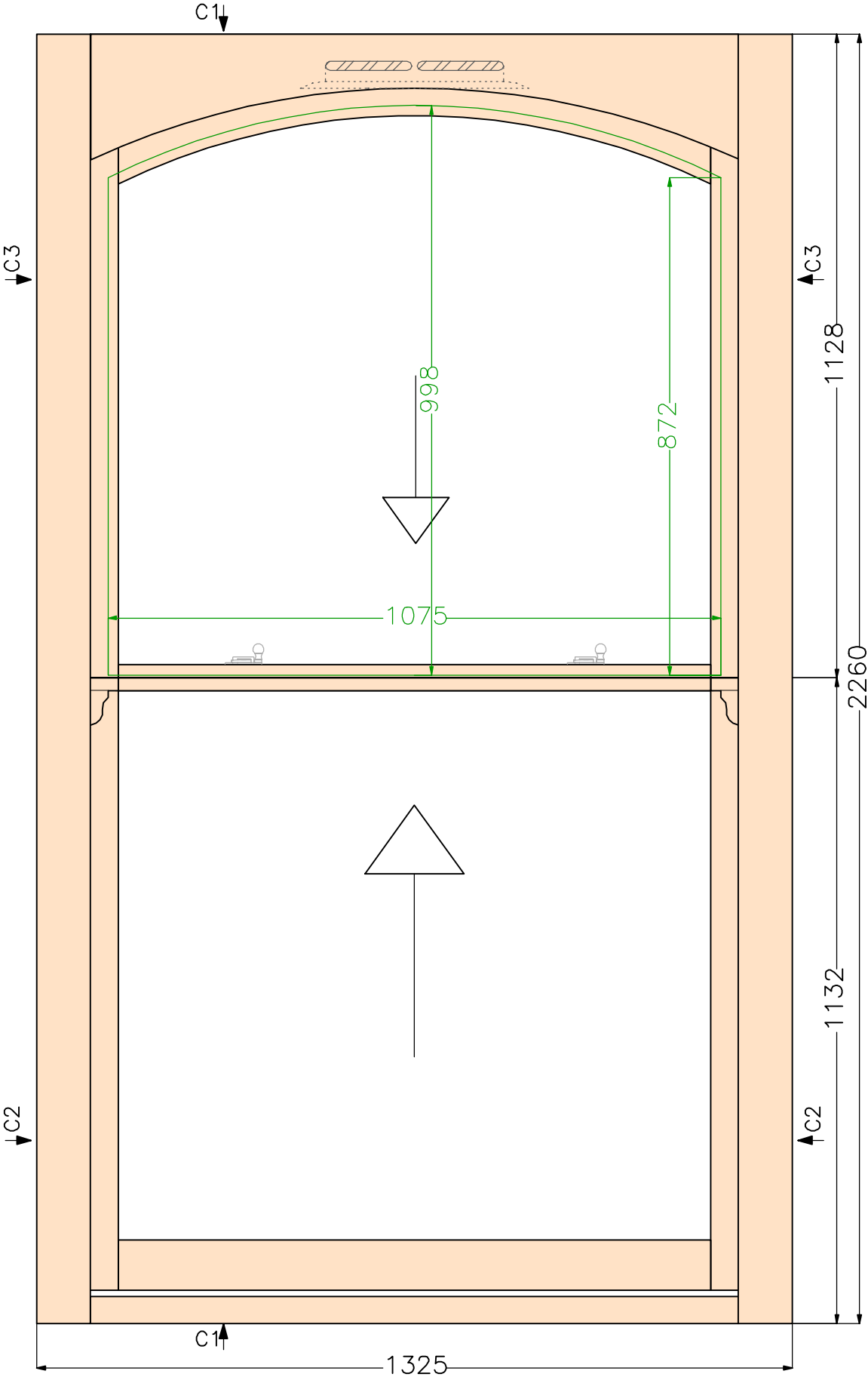
View from outside (scale 1:10)
