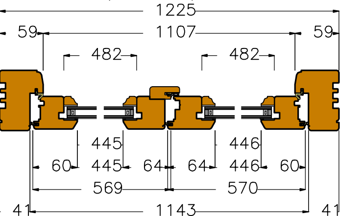
Section C2 (scale 1:5)
