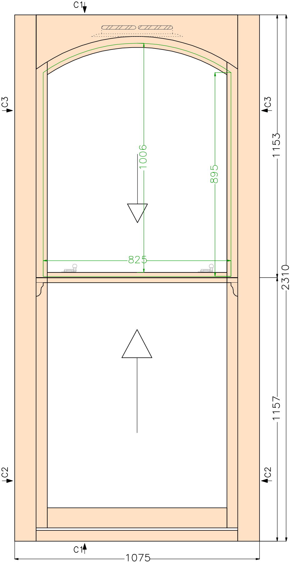
View from outside (scale 1:10)
