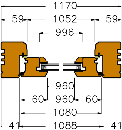
Section C3 (scale 1:5)
