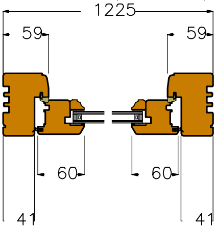
Section C3 (scale 1:5)
