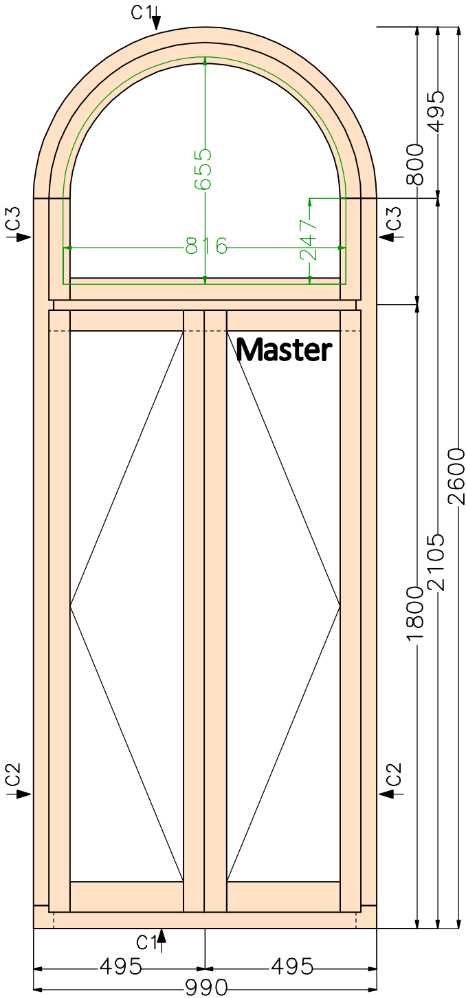
View from outside (scale 1:15)
