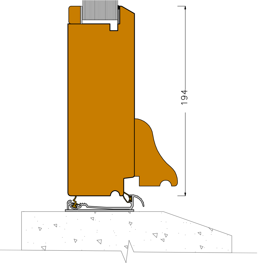
Section C7 (scale 1:2)
