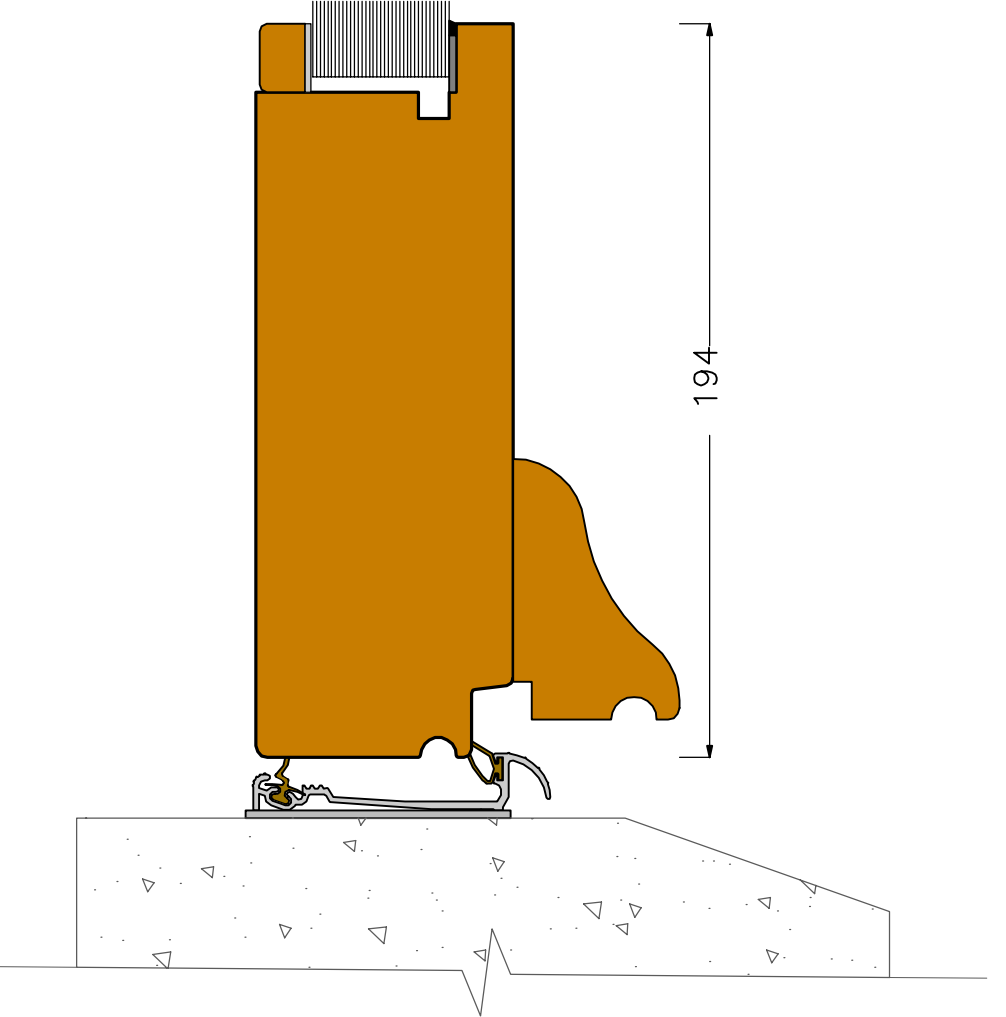
Section C8 (scale 1:2)
