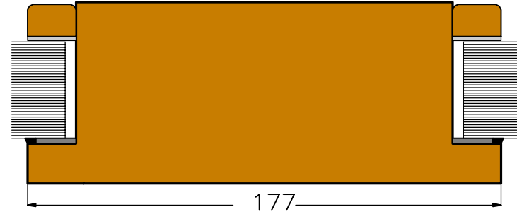
Section C12 (scale 1:2)
