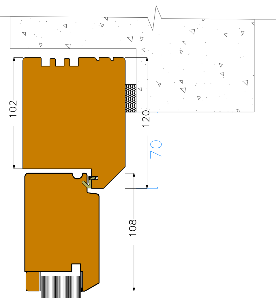
Section C4 (scale 1:2)
