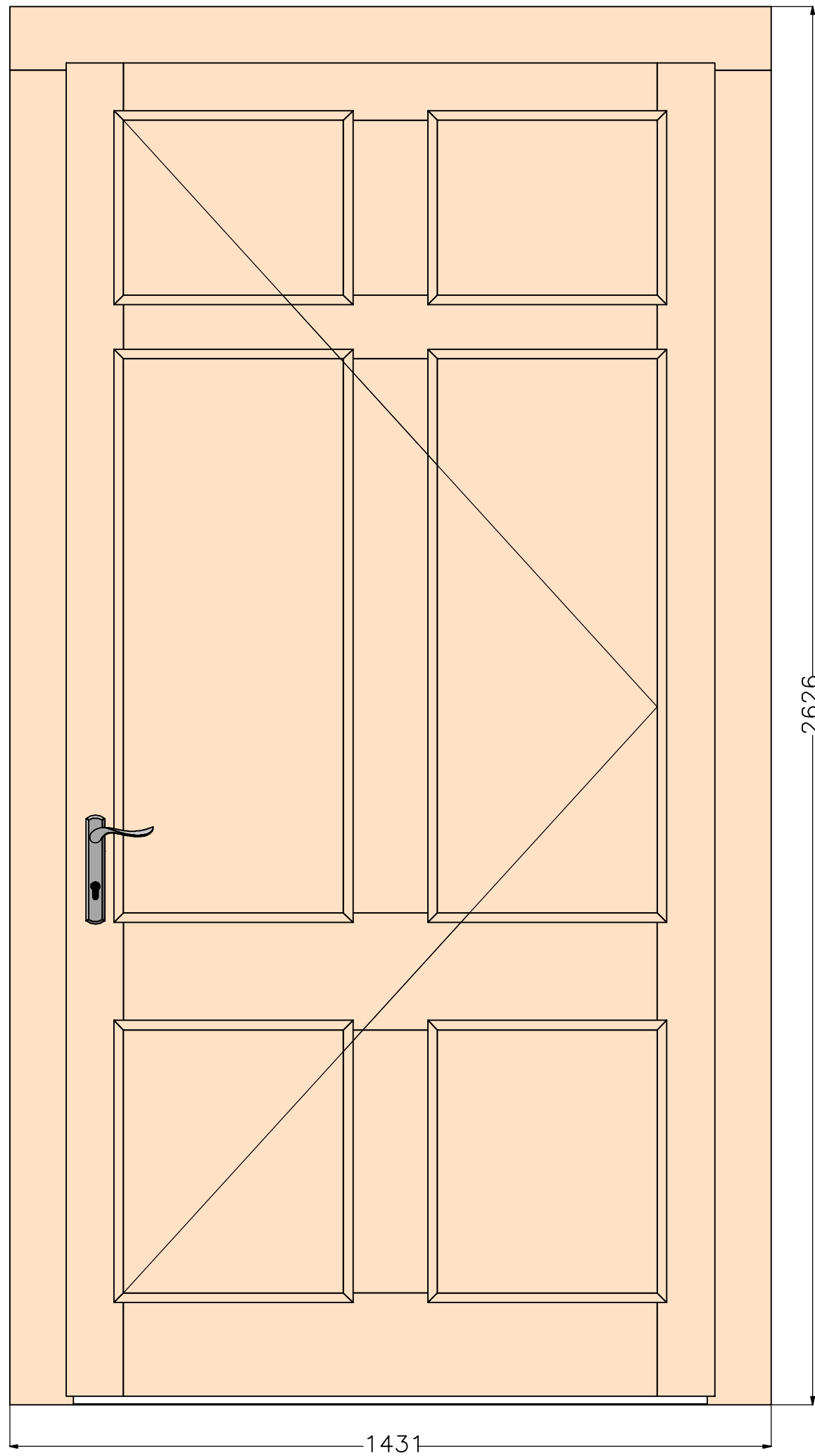
View from inside (scale 1:10)
