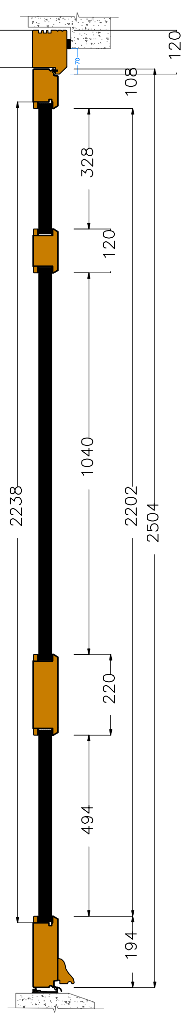
Section C1 (scale 1:10)
