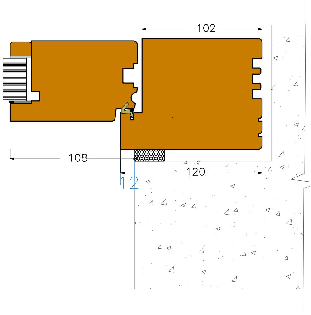
Section C9 (scale 1:2)
