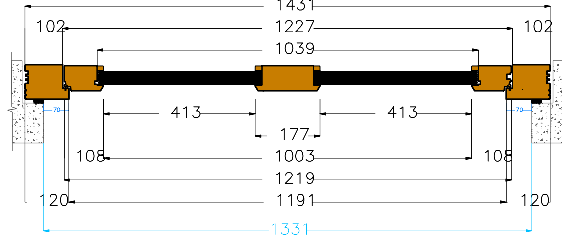
Section C2 (scale 1:10)
