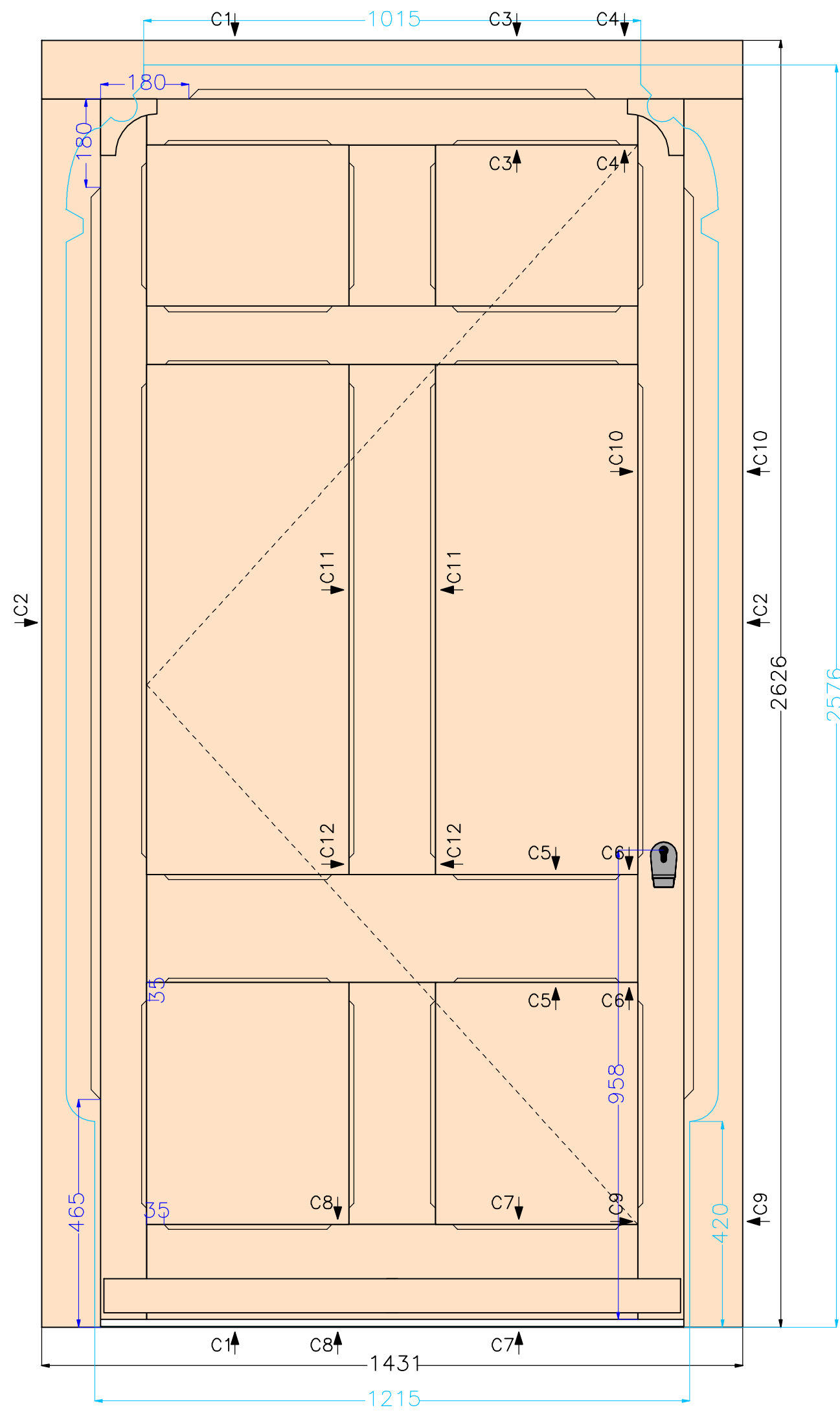
View from outside (scale 1:10)
