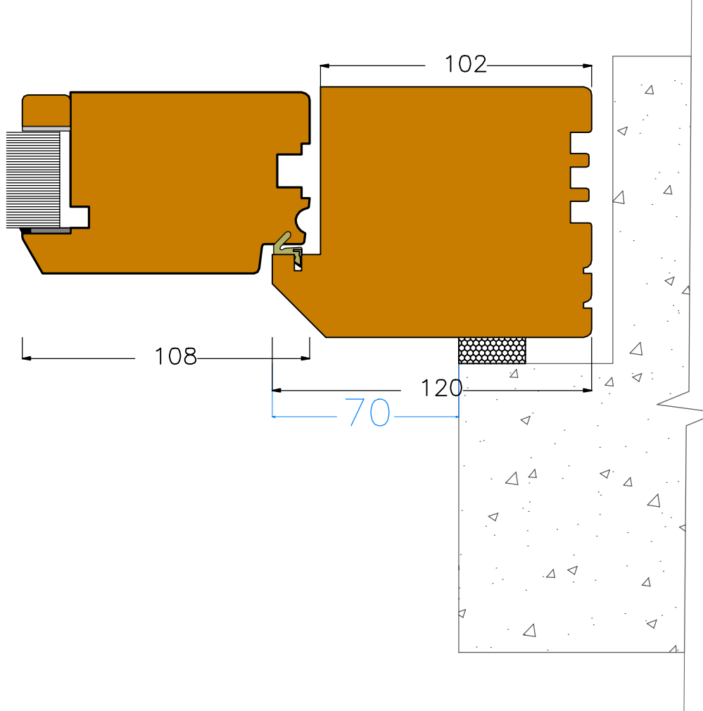
Section C10 (scale 1:2)
