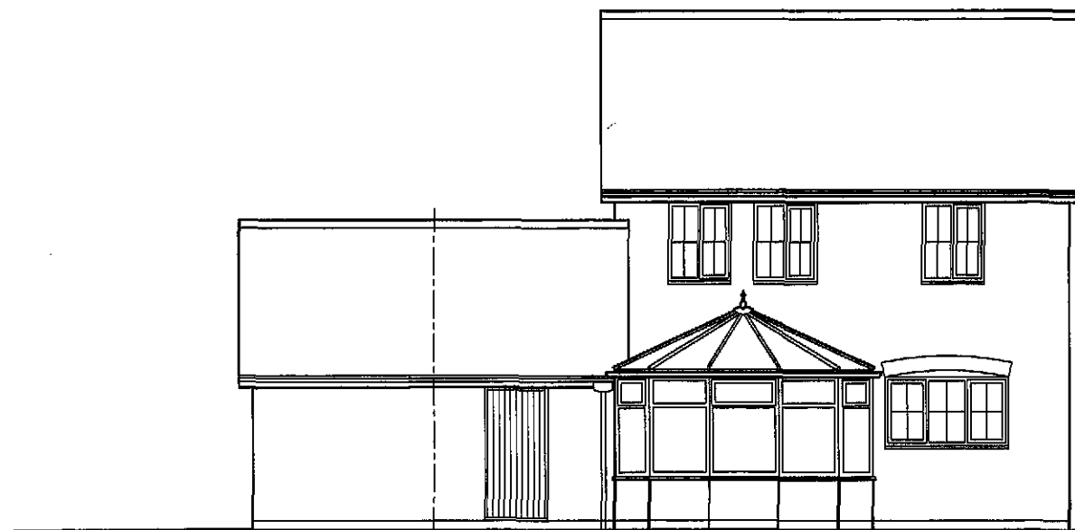
Rear Elevation (South West)
