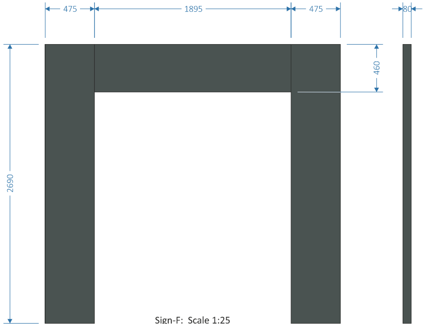
Sign-F: Scale 1:25 Folded Aluminium Panels Finished Grey Ral 7043 and Installed Around Entrance
