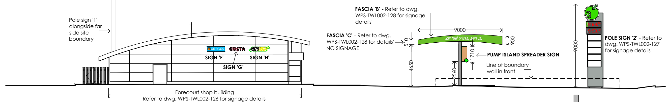
ELEVATION ACROSS FORECOURT FROM DEVELOPMENT CIRCULATION ROAD
