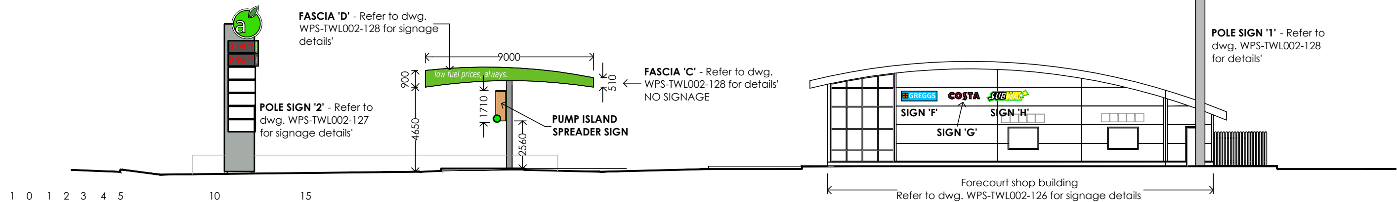
ELEVATION TO FORECOURT FROM HIGHWAY ACCESS ROAD
