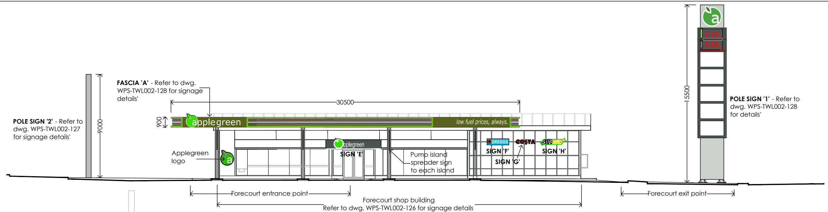
ELEVATION TO FORECOURT FROM ENTRANCE
