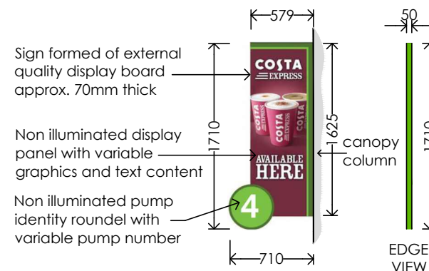
PUMP ISLAND SPREADER SIGN ELEVATION
