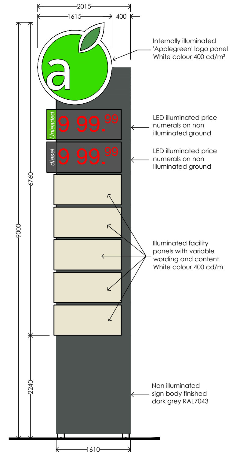
POLE SIGN '2' FACE ELEVATION
