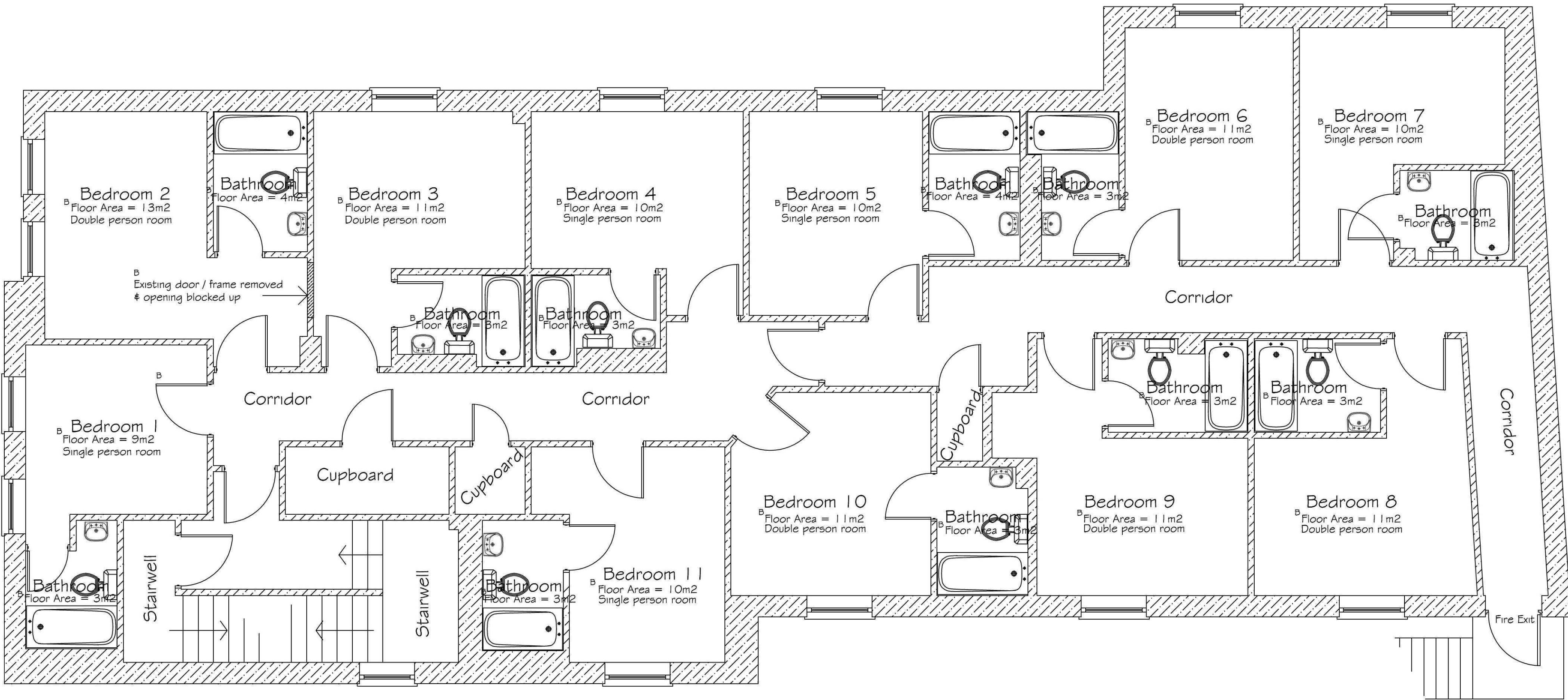
A Proposed First Floor Plan
