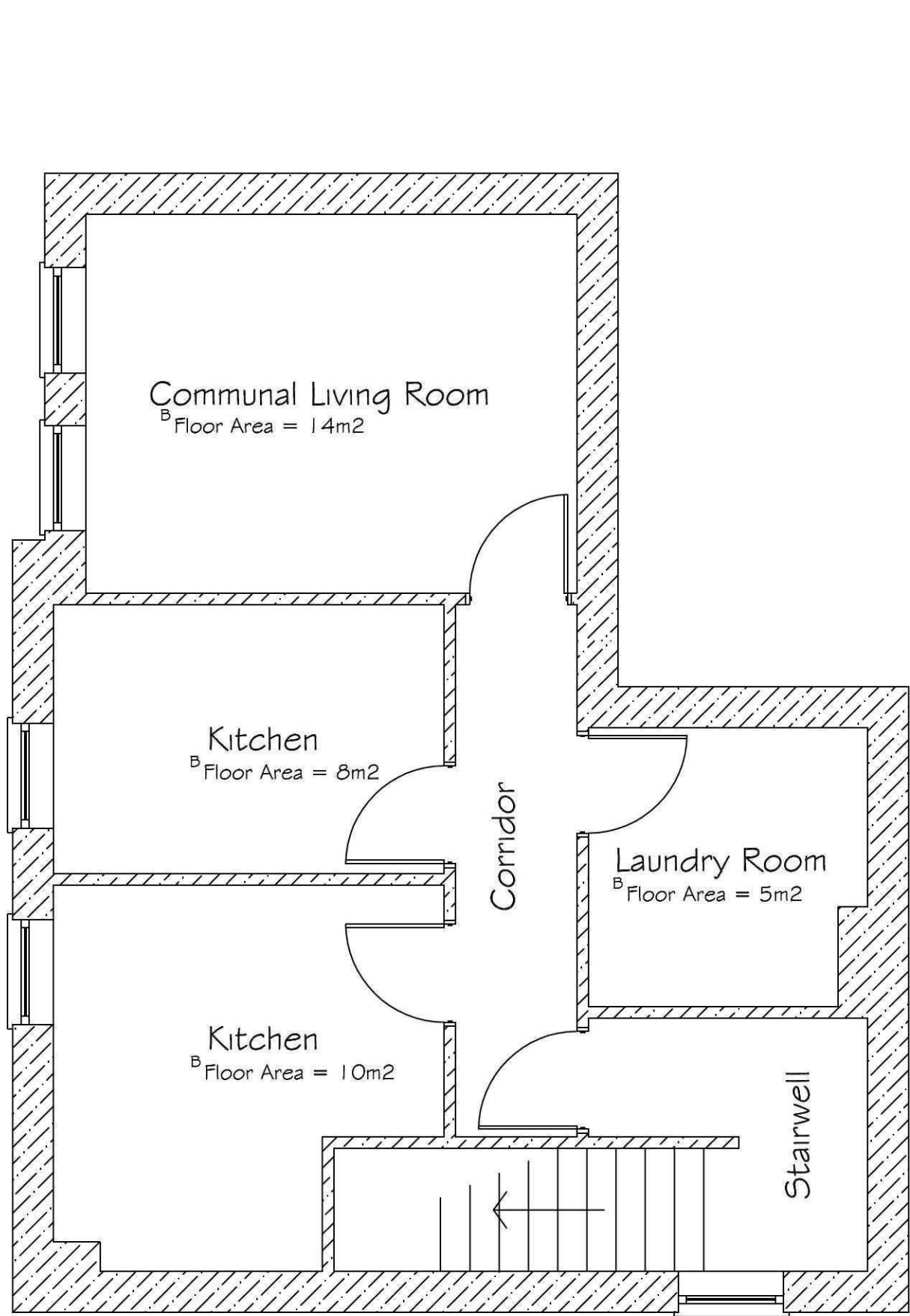
A Proposed Second Floor Plan
