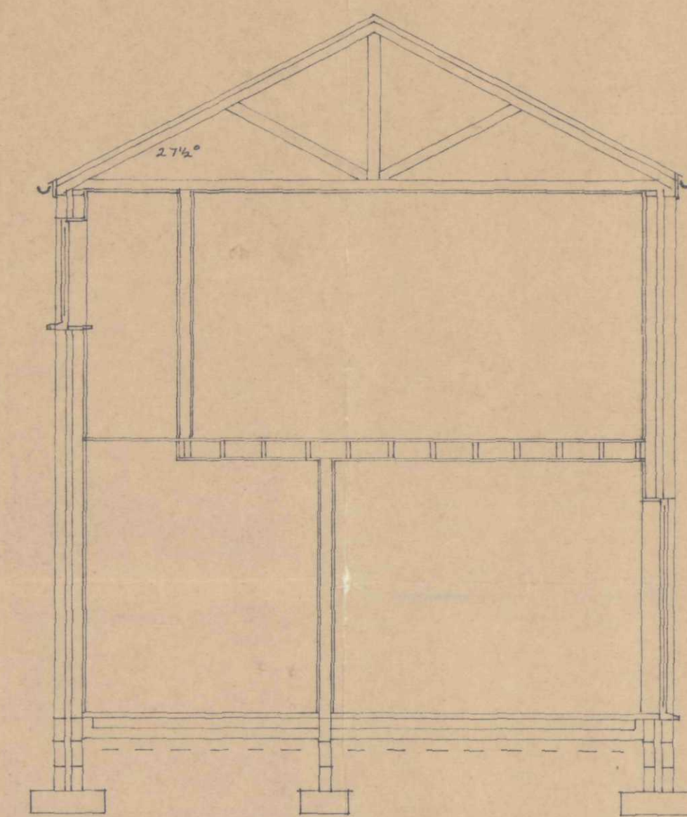
Cross Section
