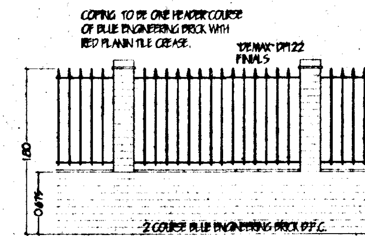
WALL/RAILING TYPICAL DETAIL. ALL TO BE 215mm THICK IN ENGLISH GARDEN WALL BOND
