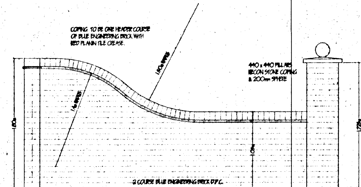
WALLING TYPICAL DETAIL. ALL TO BE 215mm THICK IN ENGLISH GARDEN WALL BOND
