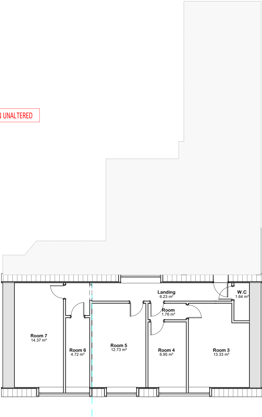
Plan 03 - 2nd Floor 1 : 100
