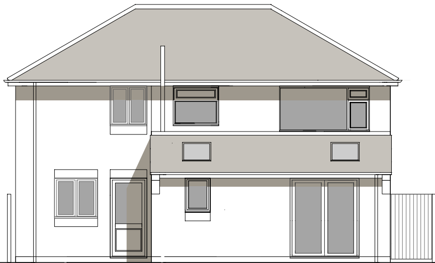
REAR ELEVATION
