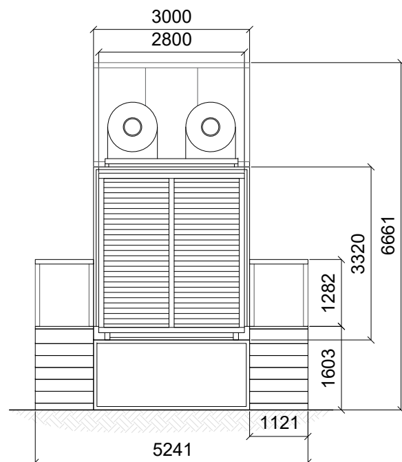
SIDE ELEVATION
