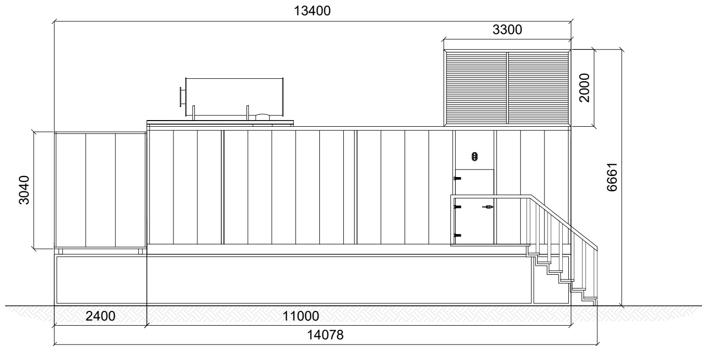
BACK ELEVATION
