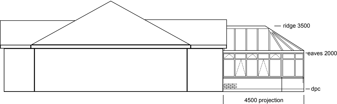
Proposed Side (South) Elevation 1:100
