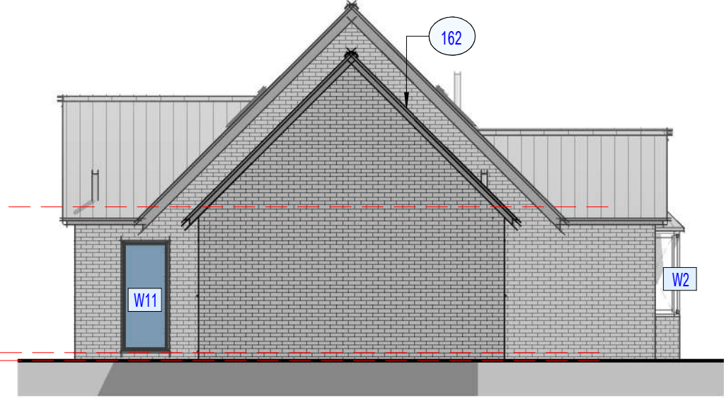
Elevation 04 - Left (east)
