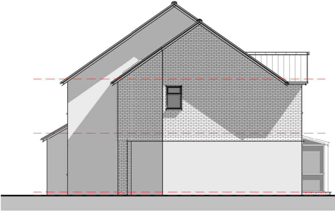
Elevation 04 – Left 1 : 100
