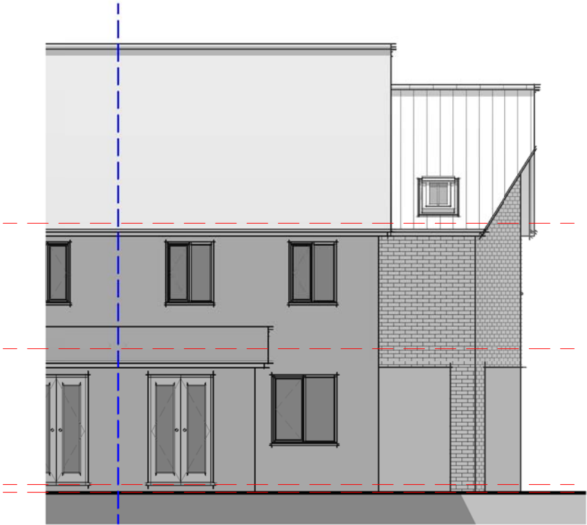
Elevation 03 – Rear 1 : 100
