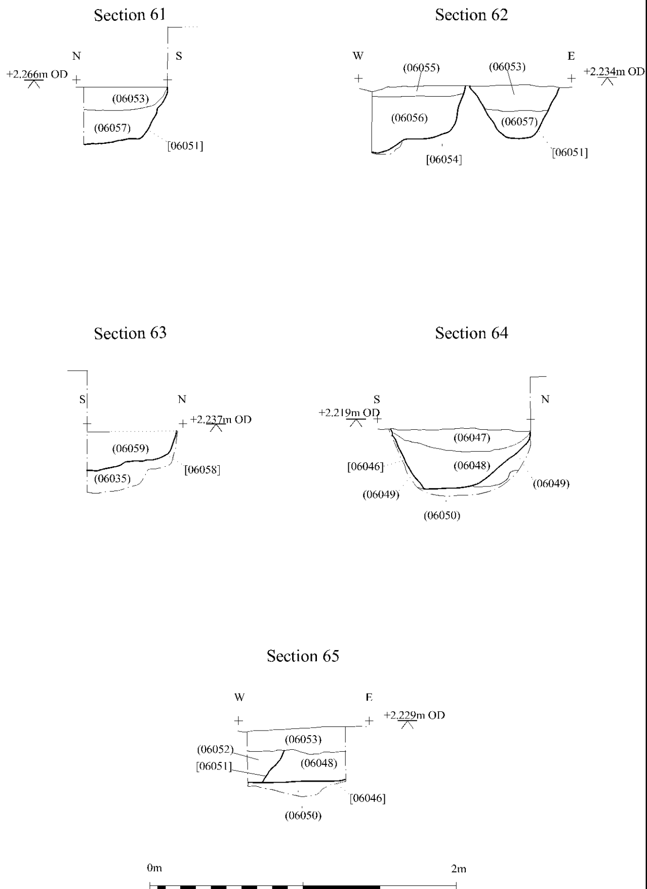
Witham Archaeology SCSP21 Trench 6 Sections 61, 62, 63, 64 & 65 Scale 1: 25 Fig. 15
