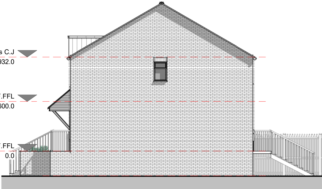
Elevation 02 – Right 1 : 100
