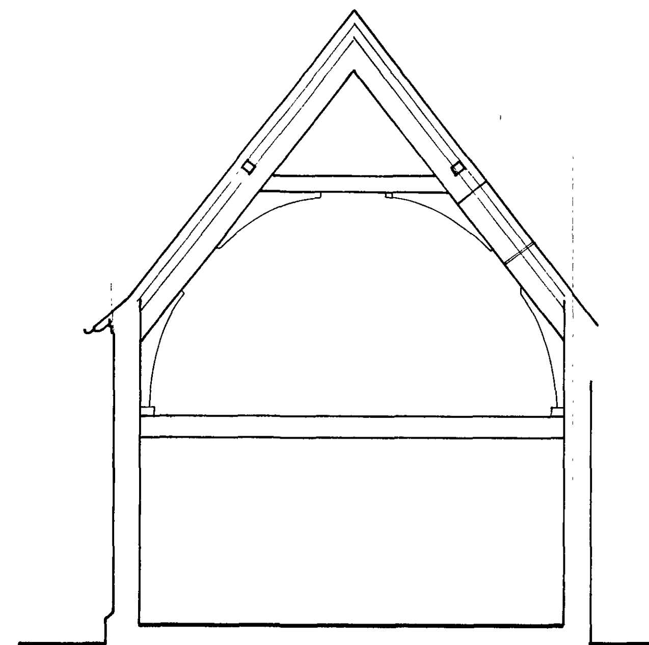
Proposed section
