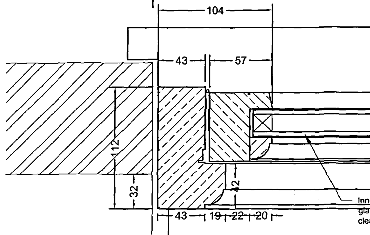
Plan Section Through Window Frame Jamb (Scale = 1 to 2)
