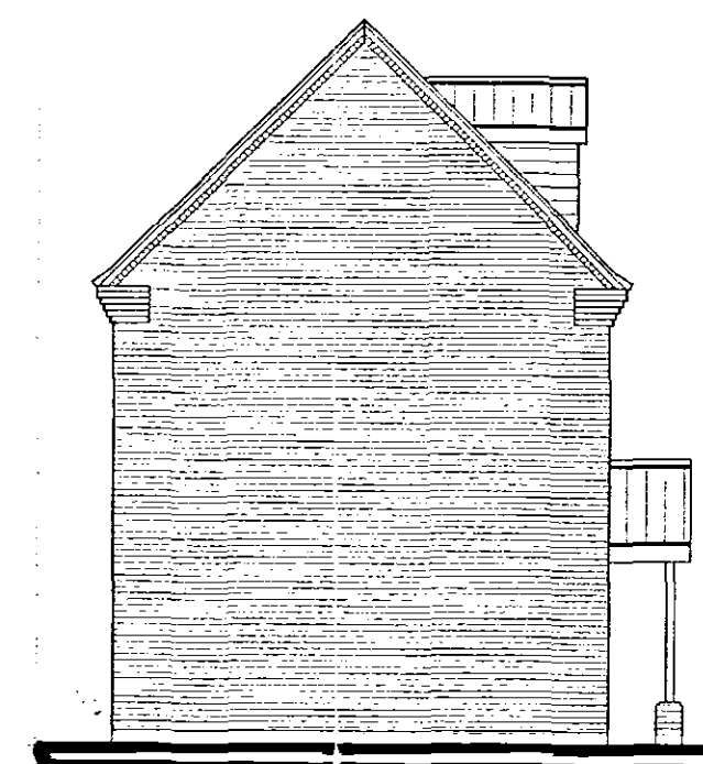
SIDE ELEVATION
