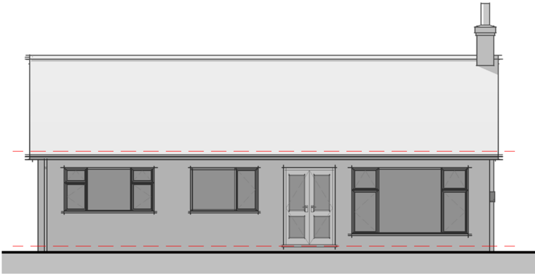
Elevation 01 - Front 1 : 100
