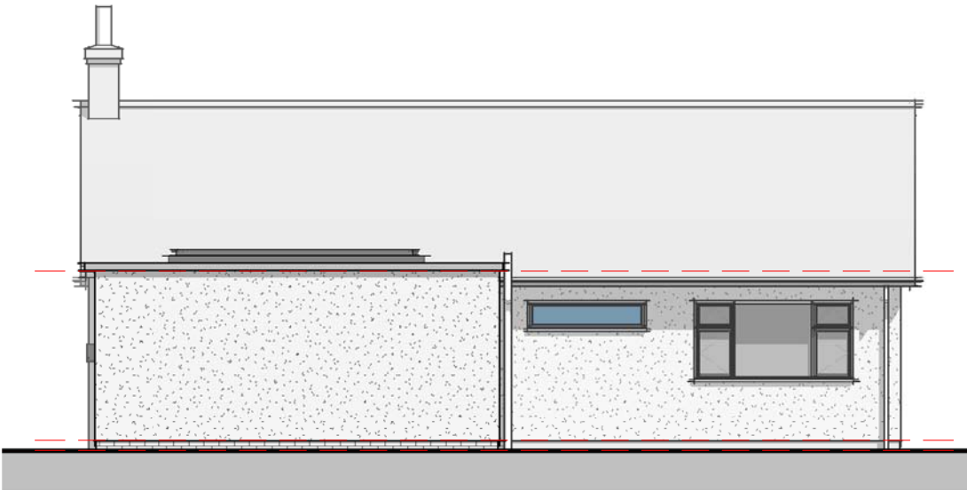
Elevation 03 - Rear 1 : 100
