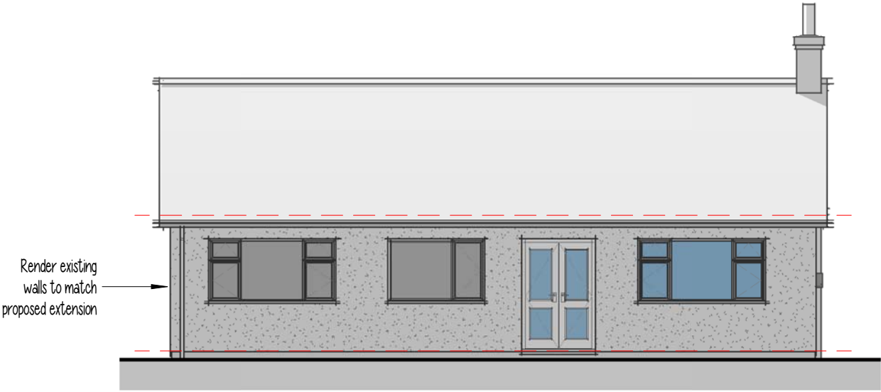
Elevation 01 - Front 1 : 100
