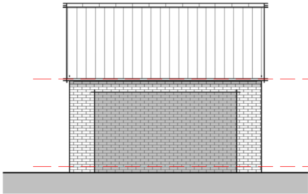
Elevation 01 - Front 1 : 100
