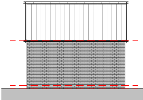
Elevation 03 - Rear 1 : 100
