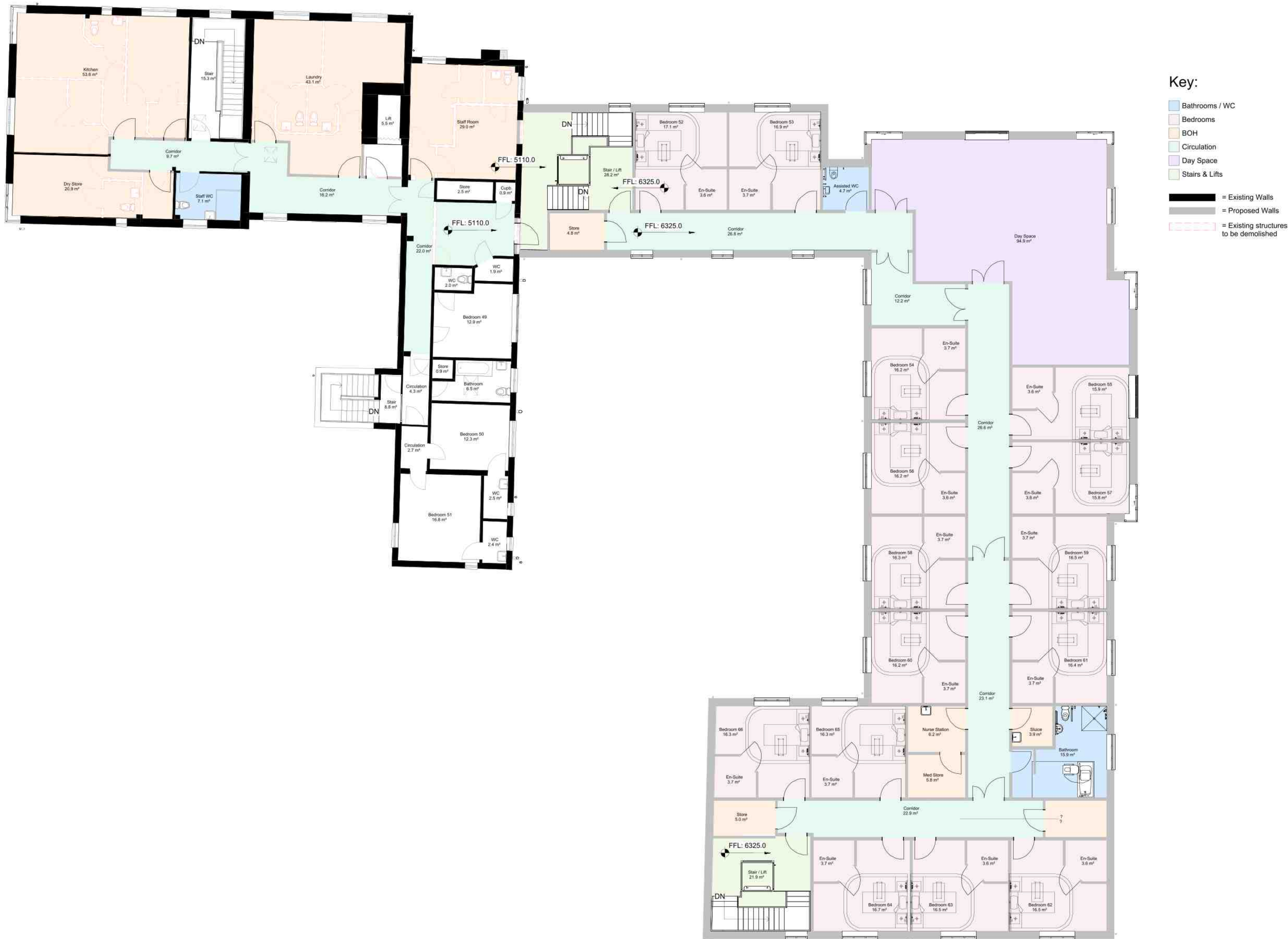
Proposed First Floor Layout 1:100
