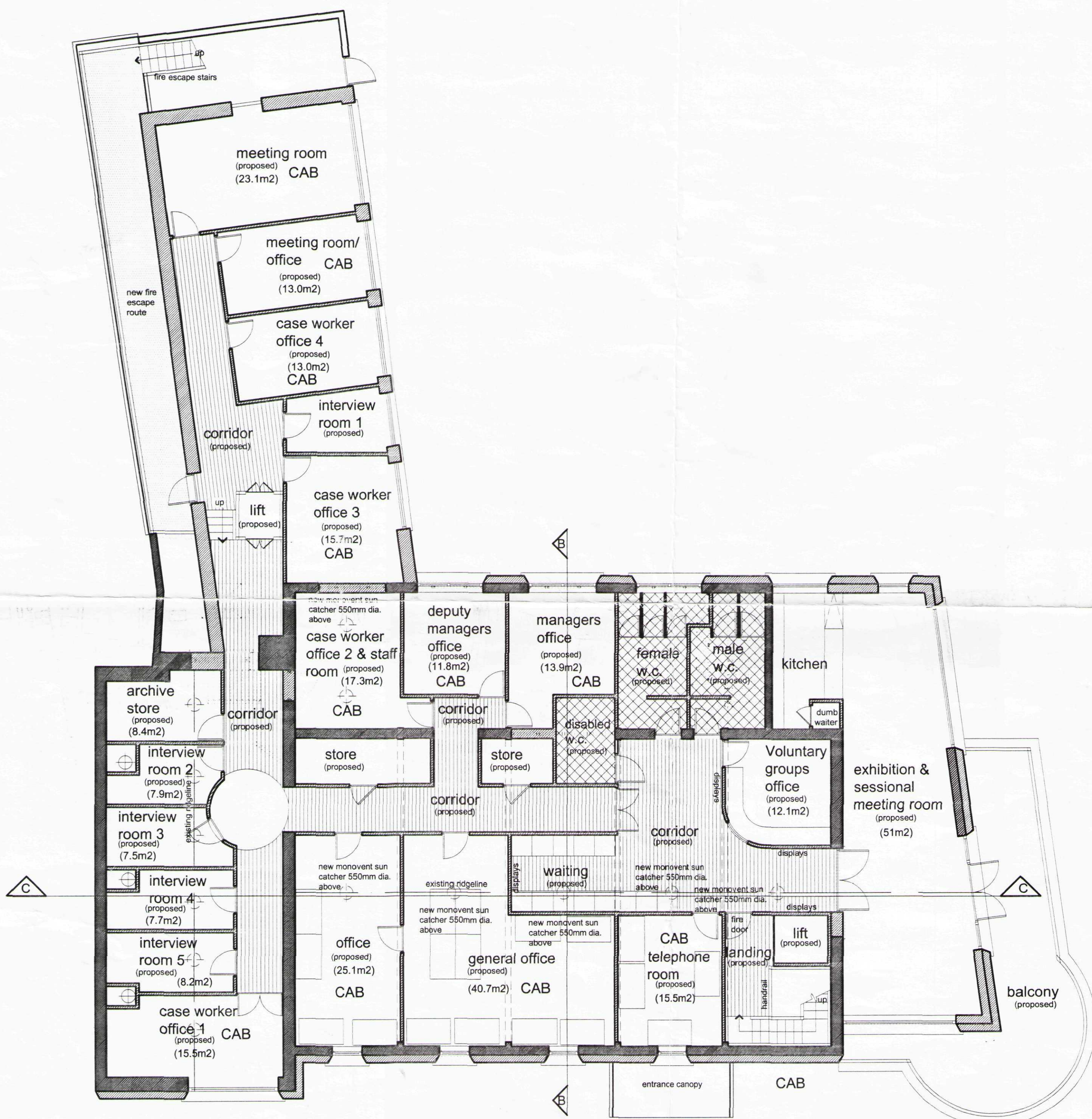
First Floor Plan 1:100
