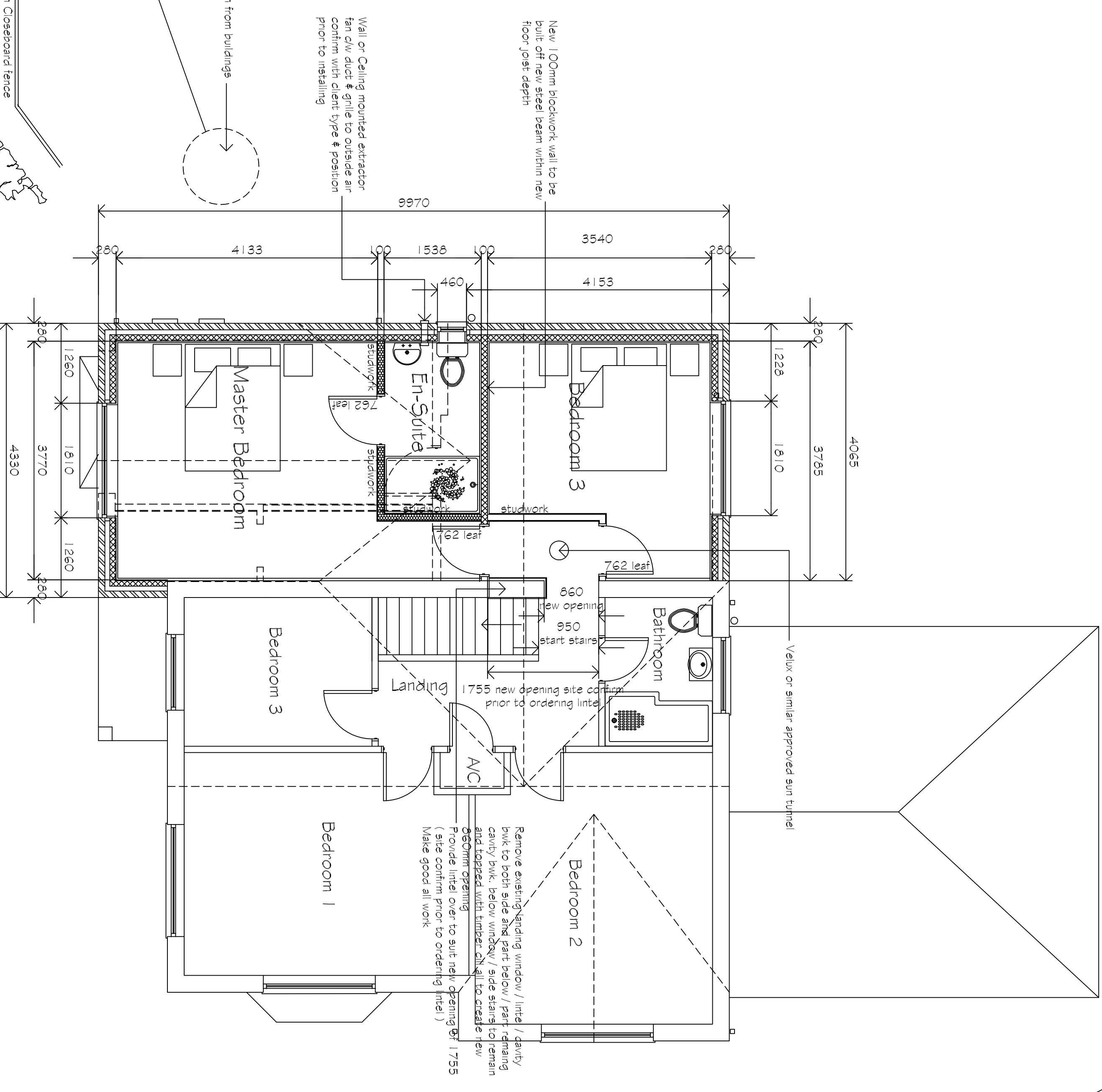
Proposed / Existing First Floor Plan Scale 1/50
