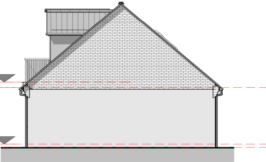
Elevation 02 – Right 1 : 100
