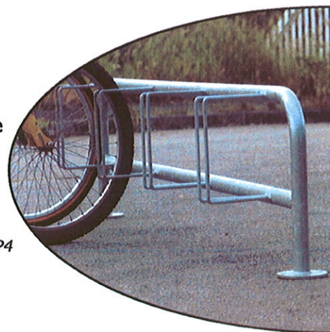
Pillar stand with holders. Also available with offset (45 degree) holders to make maximum use of available space. Accommodate up to five cycles on a single stand.
