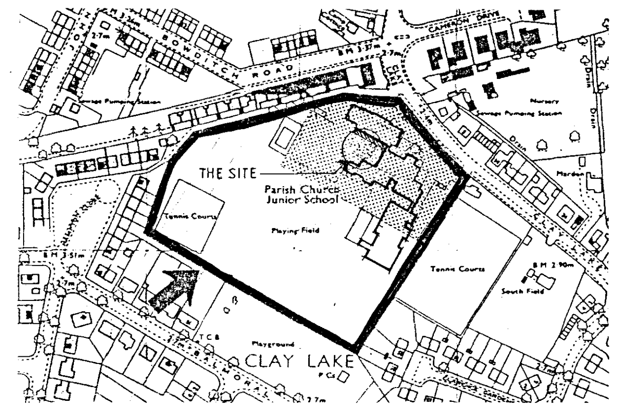
LOCATION PLAN [ 1:2500 ]
