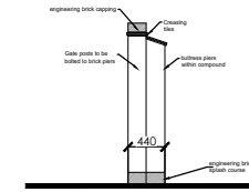
Section
