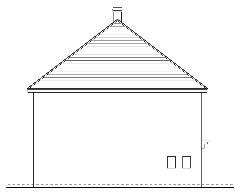
Side Elevation
