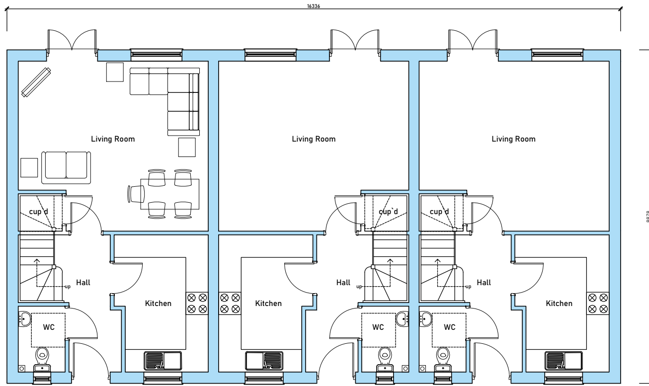
Ground floor plan (83.71m 2 / 901.08ft 2 )
