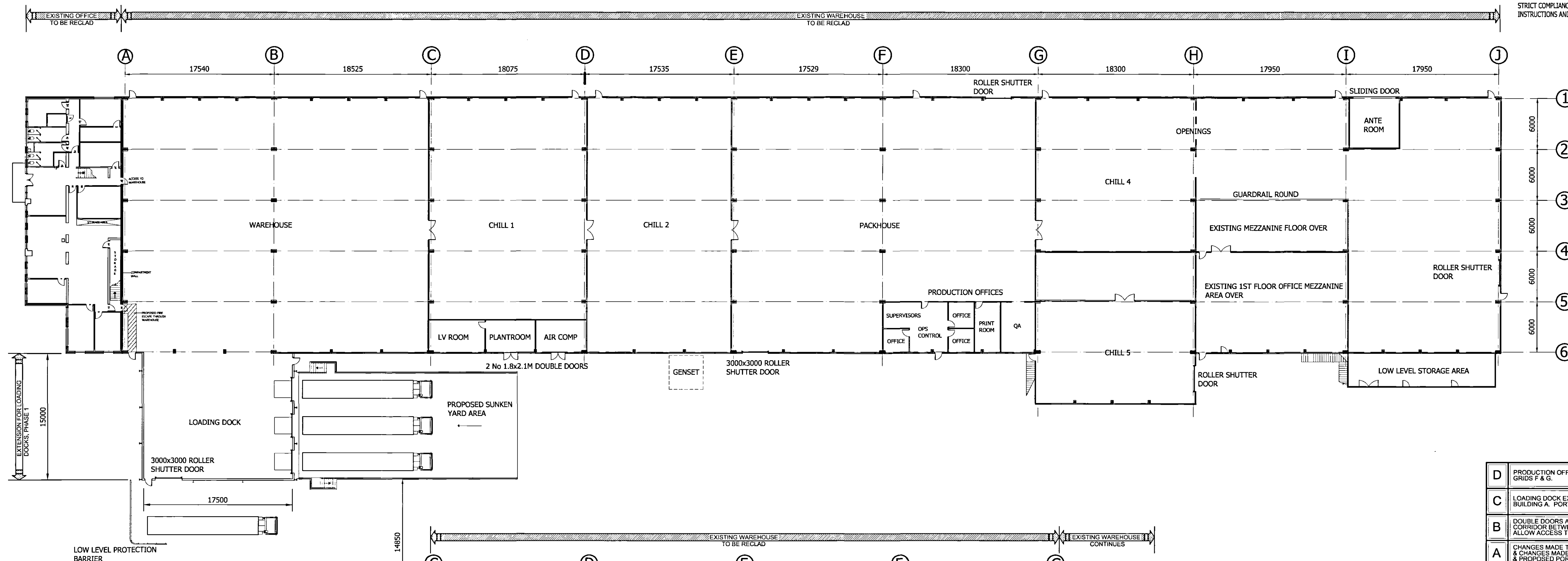
Proposed Layout - Building A (SCALE 1:250)
