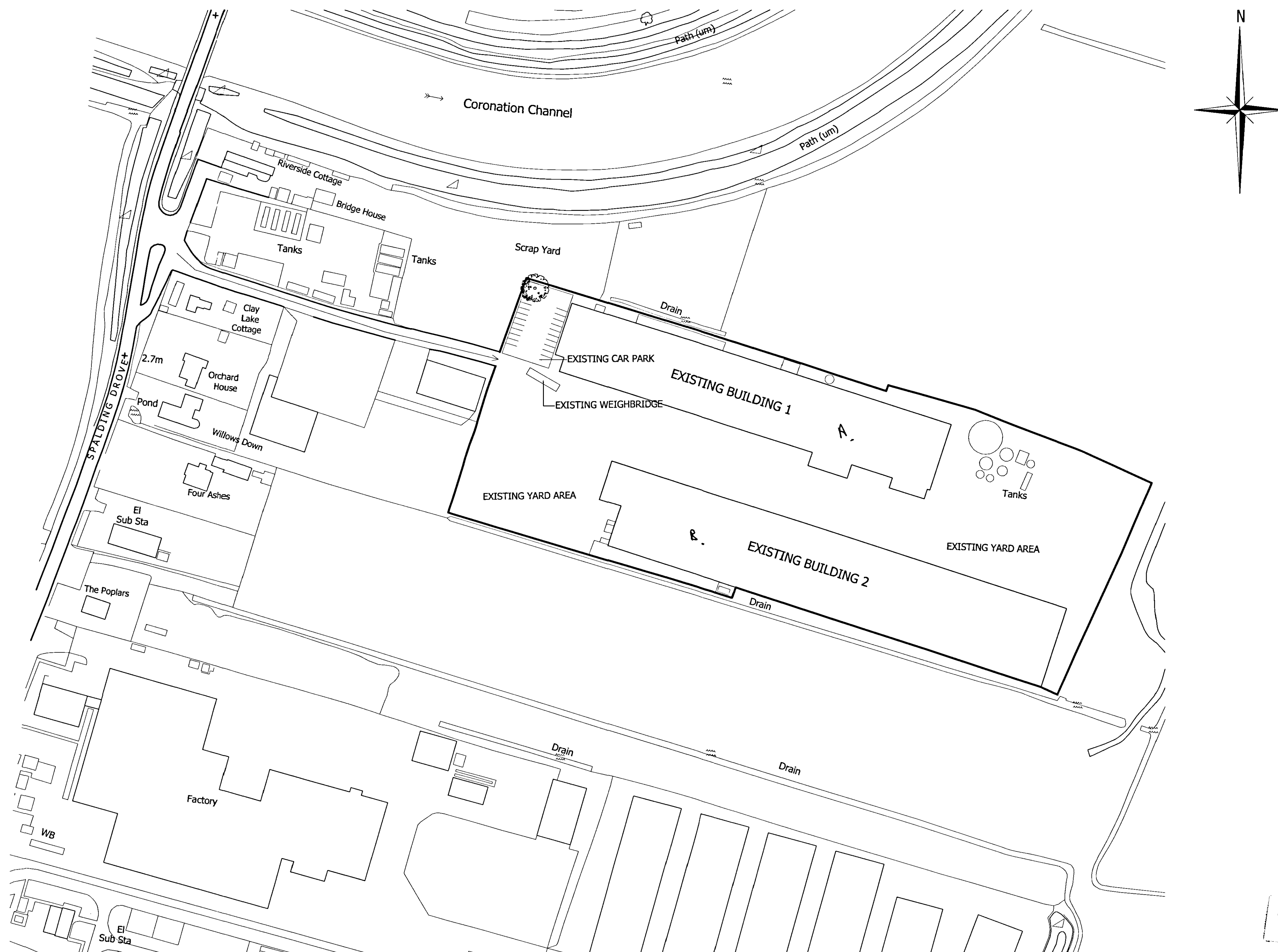
Existing Site Layout (SCALE 1:1000)
