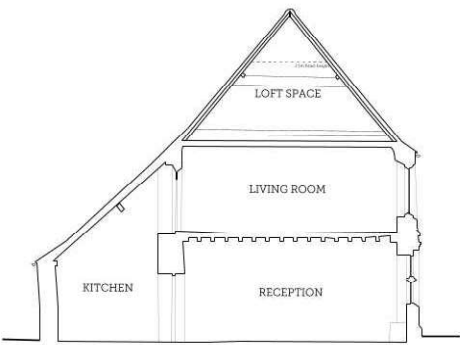
01 | EXISTING SECTION A-A Scale 1:100
