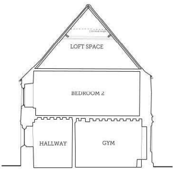
01 | EXISTING SECTION B-B Scale 1:100
