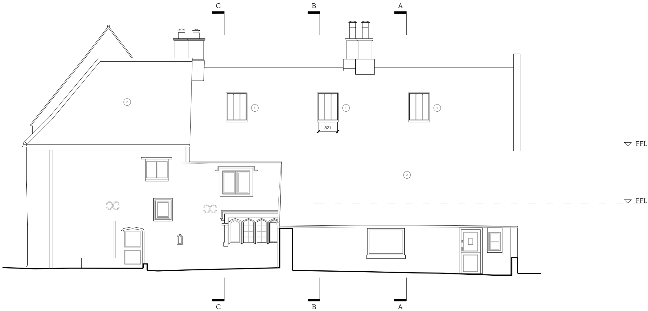
01 PROPOSED WEST ELEVATION Scale 1:100
