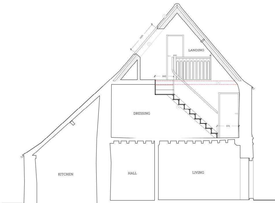
01 PROPOSED SECTION B-B Scale 1:50
