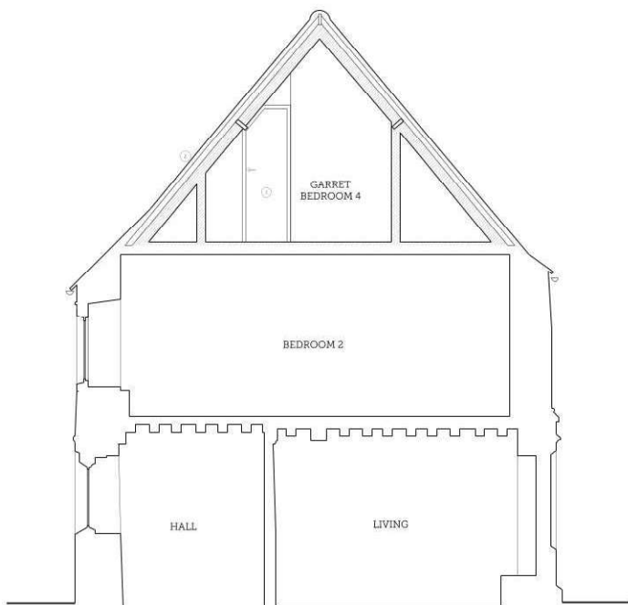
01 PROPOSED SECTION C-C Scale: 1:50
