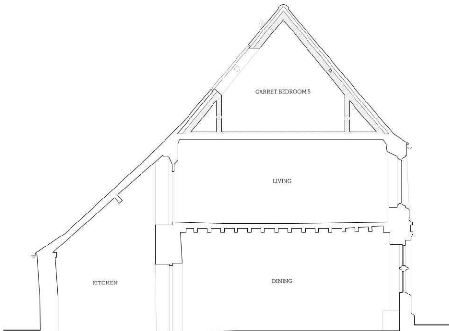
01 PROPOSED SECTION A-A Scale: 1:50
