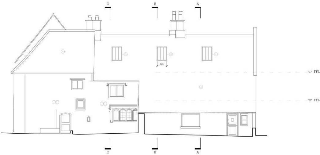
01 PROPOSED WEST ELEVATION Scale 1:100
