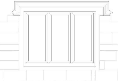
03 | EXISTING GARRET WINDOW (EAST) Scale 1:20
