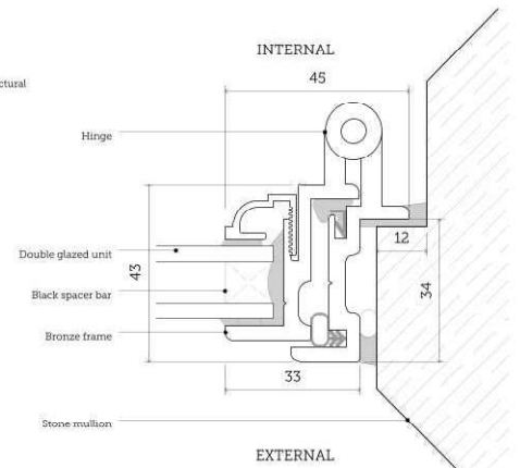
05 | PROPOSED WINDOW FRAME DETAIL Scale 1:1
