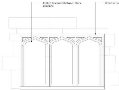
01 | EXISTING GARRET WINDOW (SOUTH) Scale 1:20
