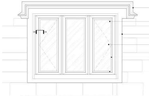
04 | PROPOSED GARRET WINDOW (EAST) Scale 1:20
