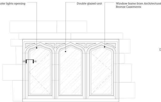
02 | PROPOSED GARRET WINDOW (SOUTH) Scale 1:20
