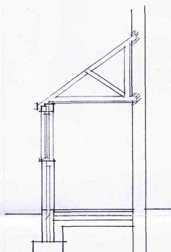
SECTION
