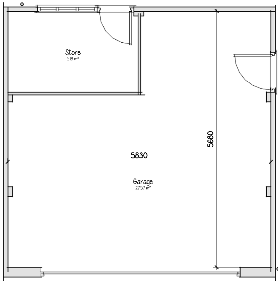
Plan 01 - Ground 1 : 50
