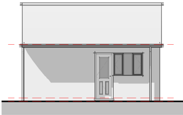
Elevation 03 - Rear 1 : 100
