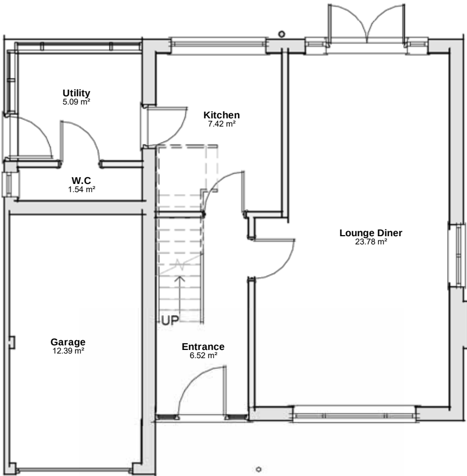
Plan 01 - Ground 1 : 75
