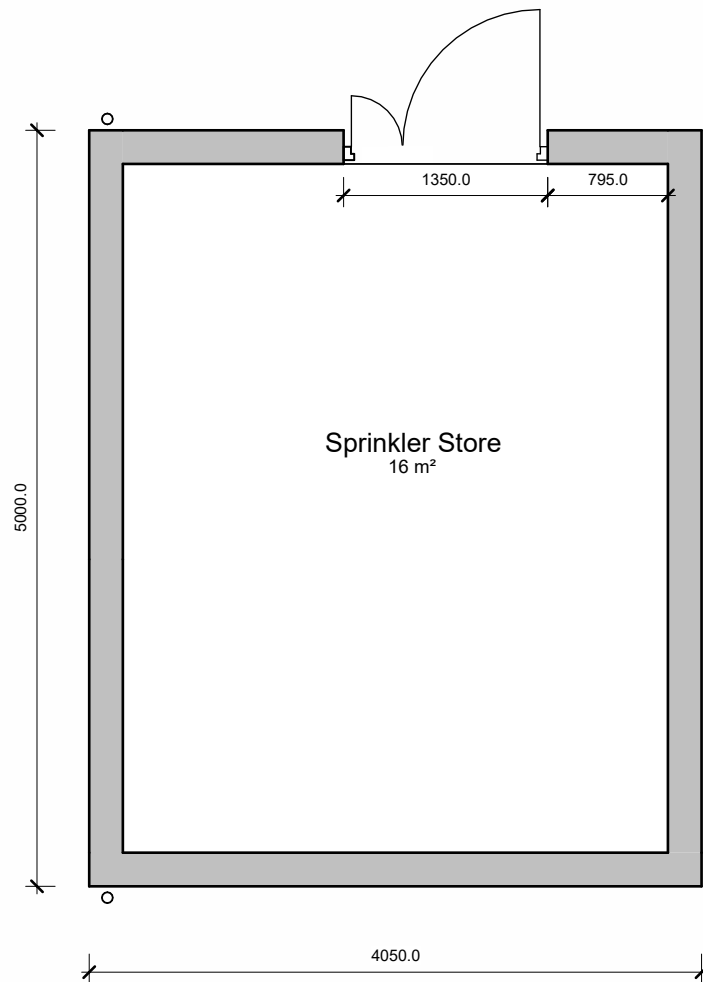
Plan View 1 : 50
