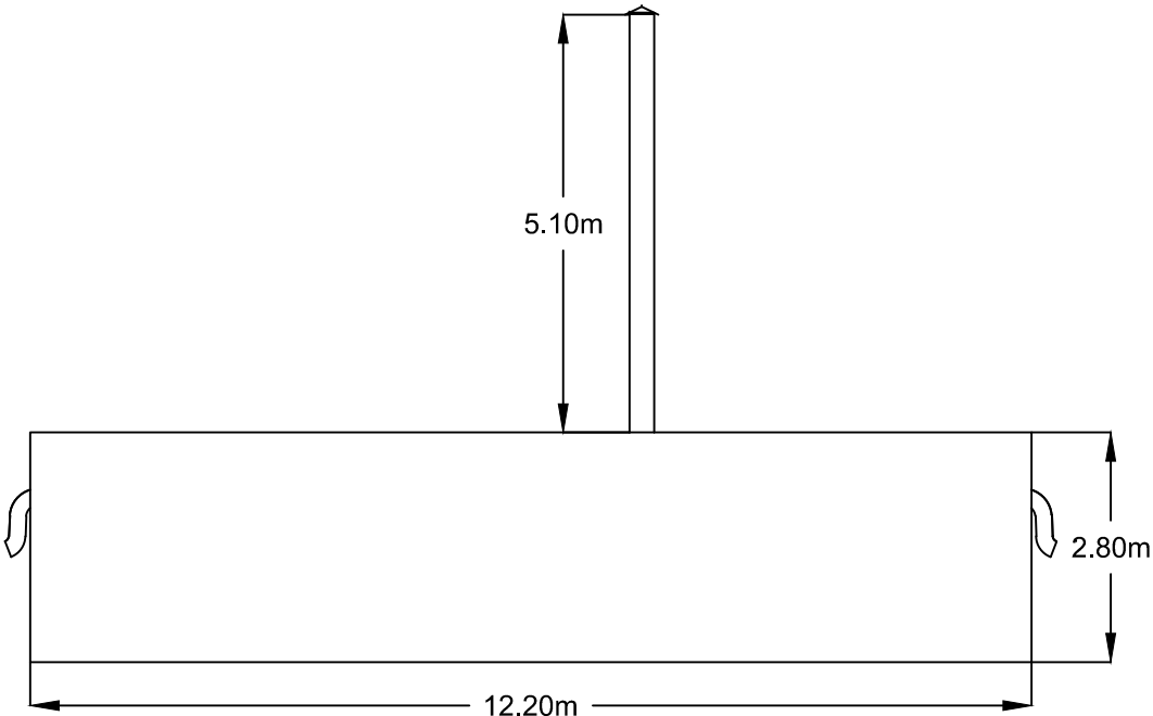
South Elevation of Bio-cabin Scale @ 1:100
