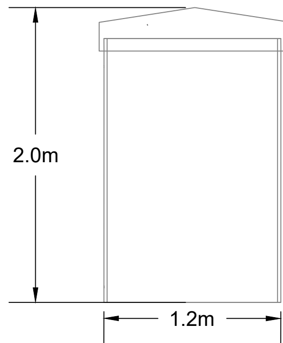
ELEVATION @ 'D'
