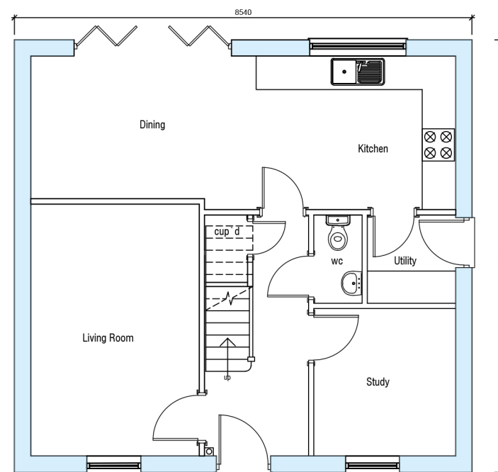
Ground Floor Layout Total Floor Area - 118.4m 2 / 1274.45ft 2
