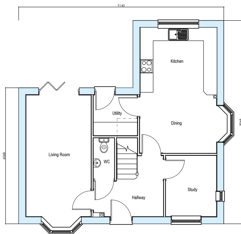
Ground Floor Plan (V2)
